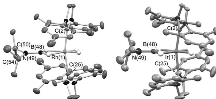
Figure 2. Structures of the cationic components of 3a (left) and 3b (right); counter-ions and hydrogen atoms (except those attached to the metal centers) omitted for clarity. Thermal ellipsoids set at the 40% probability level. Key bond lengths [Å] and angles [°]: for ( 3a ) Rh(1)···B(48) 2.204(4), B(48)–N(49) 1.370(4), Rh(1)–B(48)–N(49) 179.6(3), C(2)–Rh(1)–C(25) 165.5(1); for ( 3b ) Ir(1)···B(48) 2.088(5), B(48)–N(49) 1.379(8), Ir(1)–B(48)–N(49) 178.4(3), C(2)–Ir(1)–C(25) 165.6(2).
